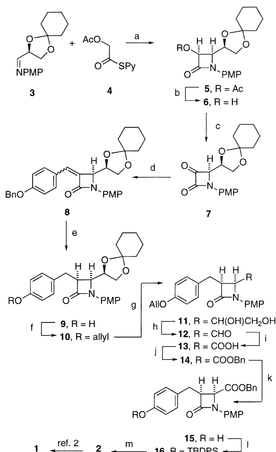
Scheme 1. Stereoselective multistep synthesis of compound 2 . Abbreviations: Py = 2-pyridyl; PMP: 4-MeOPh; All: \text{CH}_2=\text{CH}-\text{CH}_2 ; TBDPS: t -BuPh 2 Si. Reagents: (a) \text{TiCl}_4 , \text{Et}_3\text{N} ; (b) \text{KOH} ; (c) \text{P}_2\text{O}_5 , DMSO; (d) 4-BnOPh \text{CH}_2\text{PPh}_3 Br, BuLi; (e), \text{H}_2 , 10% Pd/C; (f) \text{AlI}_3 , \text{K}_2\text{CO}_3 ; (g) TFA, \text{H}_2\text{O} ; (h) \text{NaIO}_4 ; (i) Jones reagent; (j) BnBr, \text{K}_2\text{CO}_3 ; (k) \text{PdOAc}_2 , \text{PPh}_3 ; then wet \text{SiO}_2 ; (l) TBDPSCl, imidazole; (m) \text{Ce}(\text{NH}_4)_2(\text{NO}_3)_6 .
